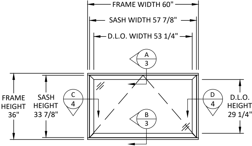
TYPICAL ELEVATION
