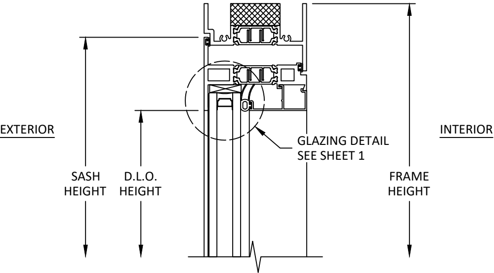
A 3 VERTICAL SECTION HEAD
