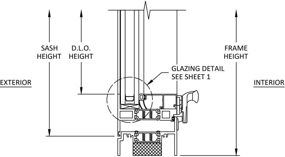
B 3 VERTICAL SECTION SILL
