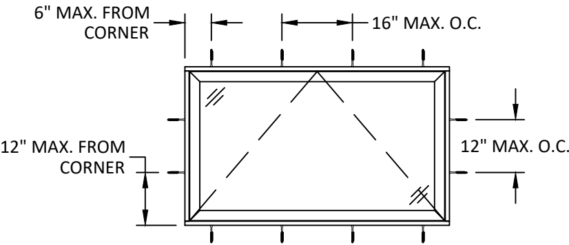
ANCHOR LAYOUT
