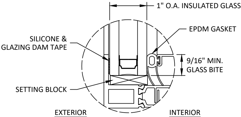
GLAZING DETAIL
